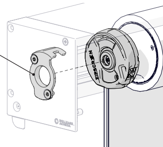
SPRING
