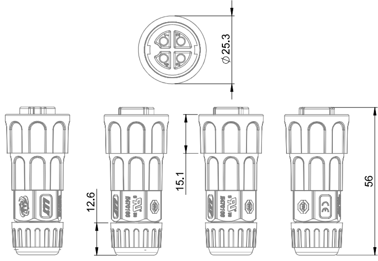
FEMALE CONNECTOR
