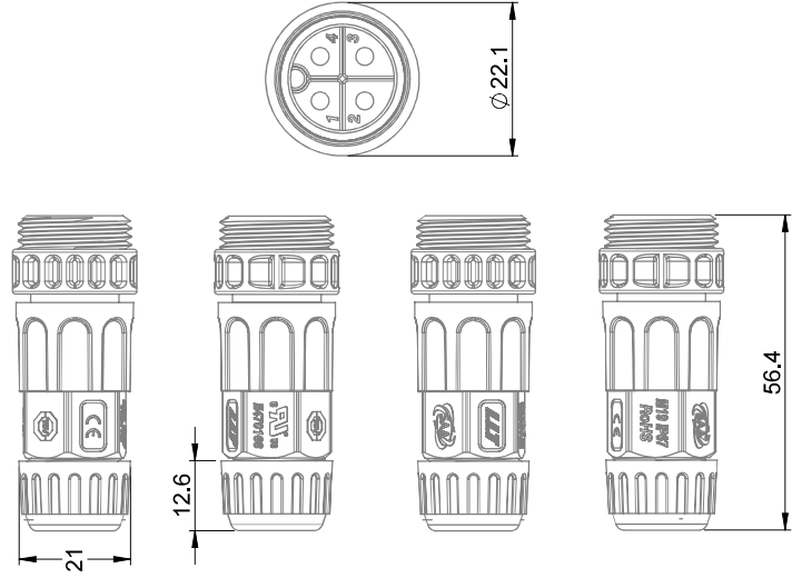
MALE CONNECTOR
